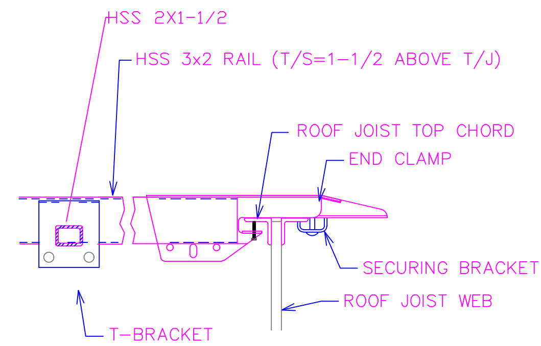
SECTION 1
