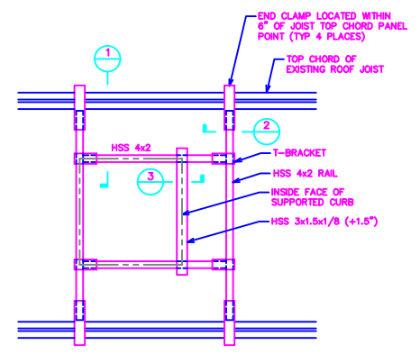
ROOF CURB FRAMING PLAN D TOP OF STEEL = TOP OF JOISTS UNLESS NOTED
