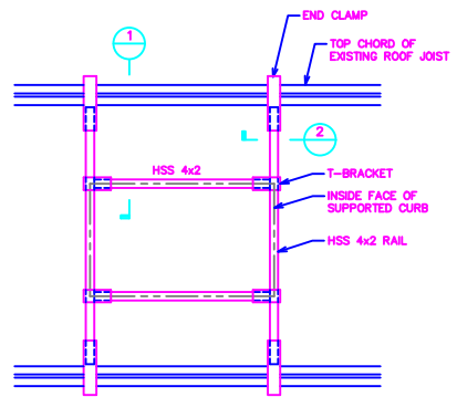
ROOF CURB FRAMING PLAN A TOP OF STEEL = TOP OF JOISTS
